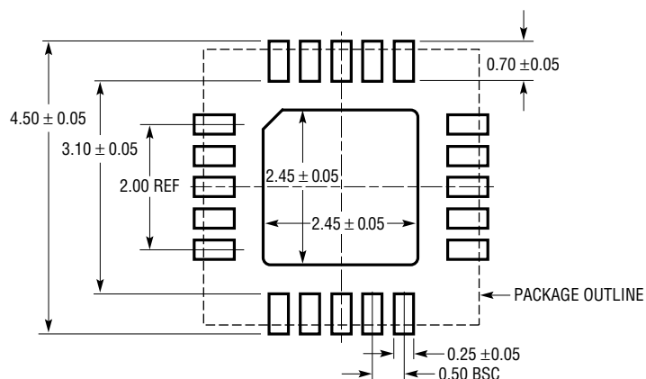
UF Package 20-Lead (4mm × 4mm) Plastic QFN (Reference LTC DWG # 05-08-1710 Rev A)
